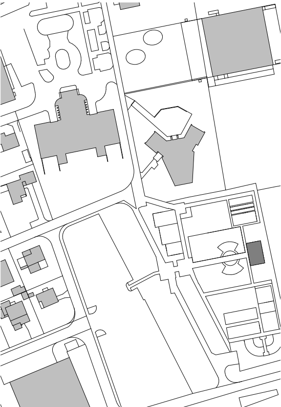
Situationsplan 1:2000
